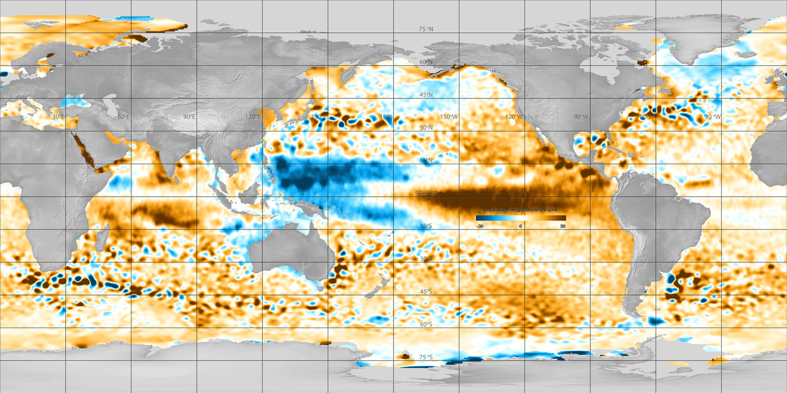
Mapping Sea Surface Height Deviation – January 2016
